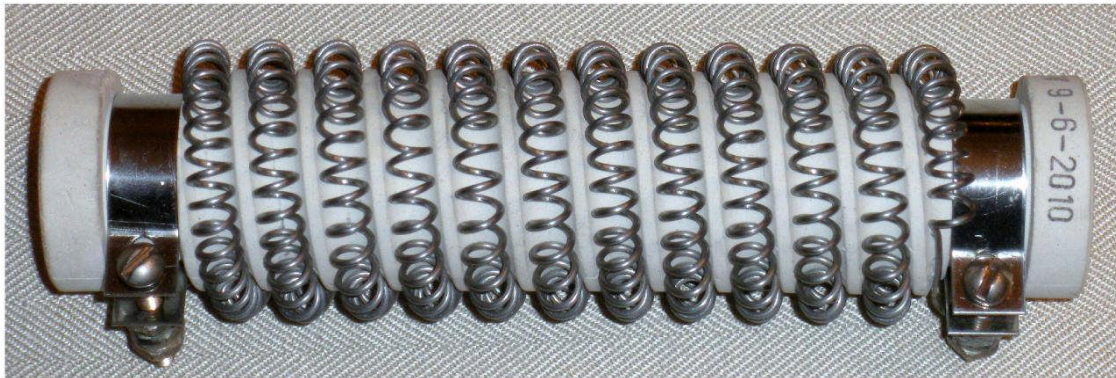
10/32 Screw Terminals with 3/8" Diameter Center Hole, 1.875" OD x 7 1/4" Long
